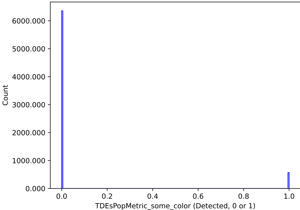
baseline_v3.3_10yrs : TDEsPopMetric_some_color
