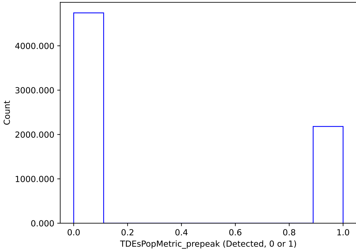
baseline_v3.3_10yrs : TDEsPopMetric_prepeak
