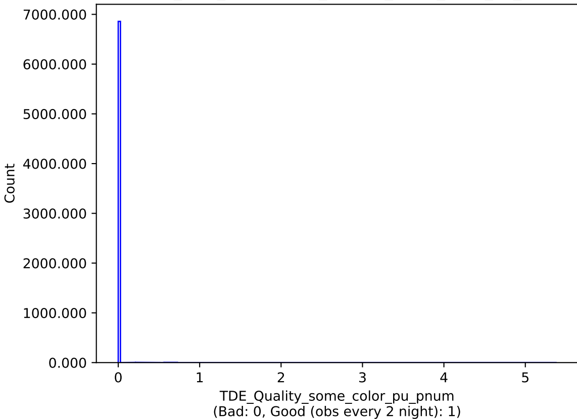
baseline_v3.3_10yrs : TDE_Quality_some_color_pu_pnum
