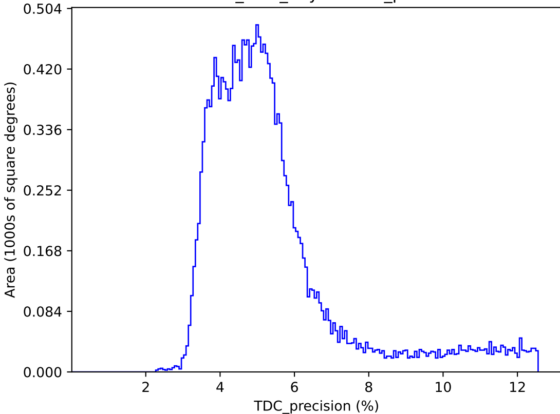
baseline_v3.3_10yrs : TDC_precision
