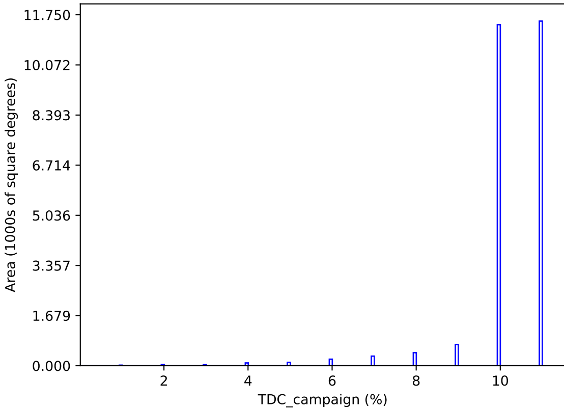
baseline_v3.3_10yrs : TDC_campaign
