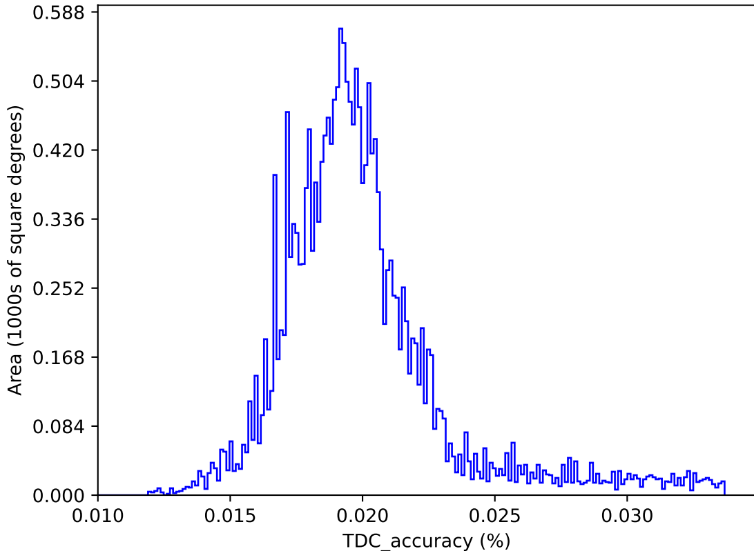
baseline_v3.3_10yrs : TDC_accuracy
