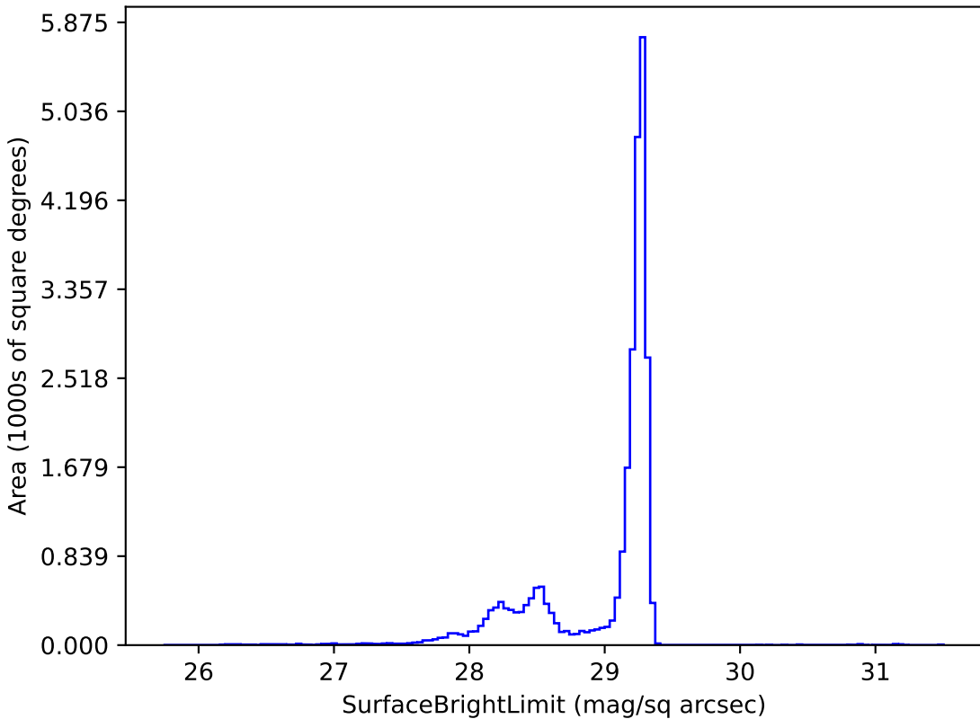
baseline_v3.3_10yrs z: SurfaceBrightLimit
