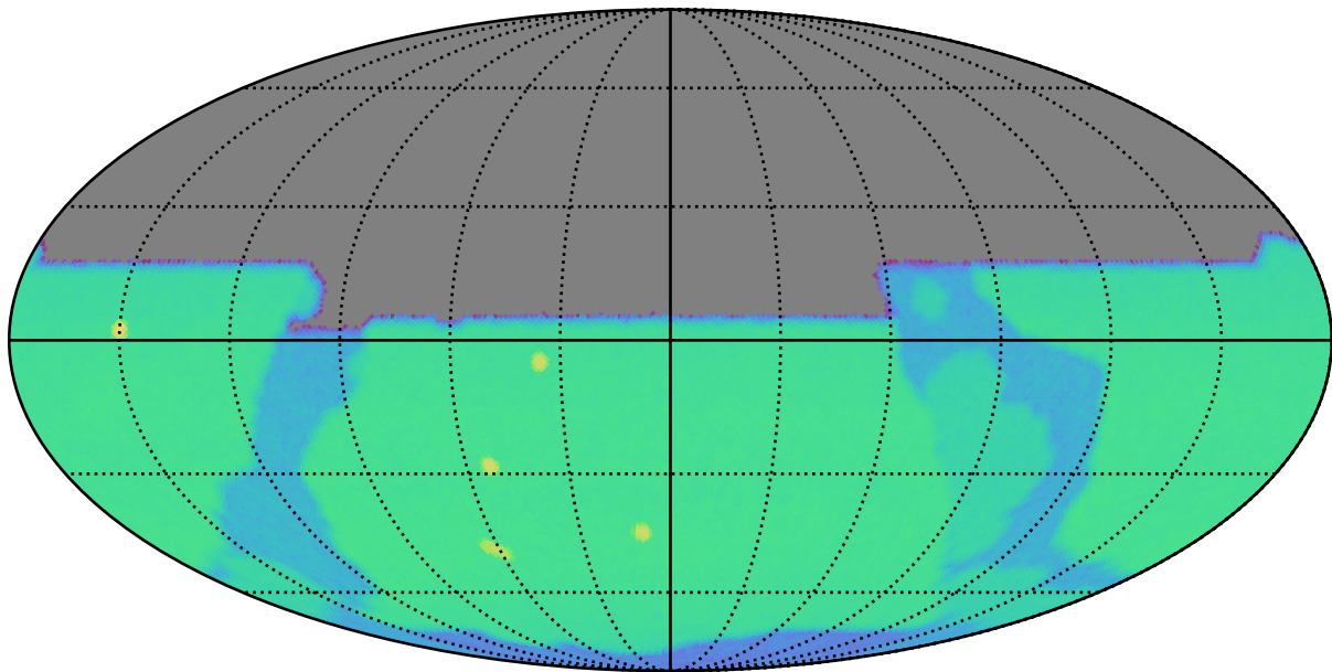
baseline_v3.3_10yrs y: SurfaceBrightLimit
