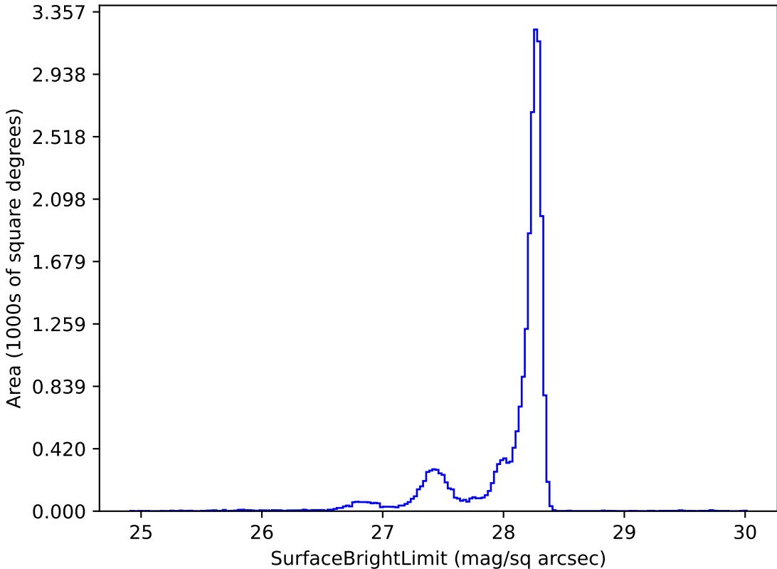
baseline_v3.3_10yrs y: SurfaceBrightLimit
