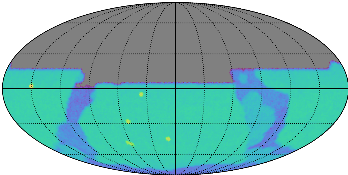
baseline_v3.3_10yrs u: SurfaceBrightLimit
