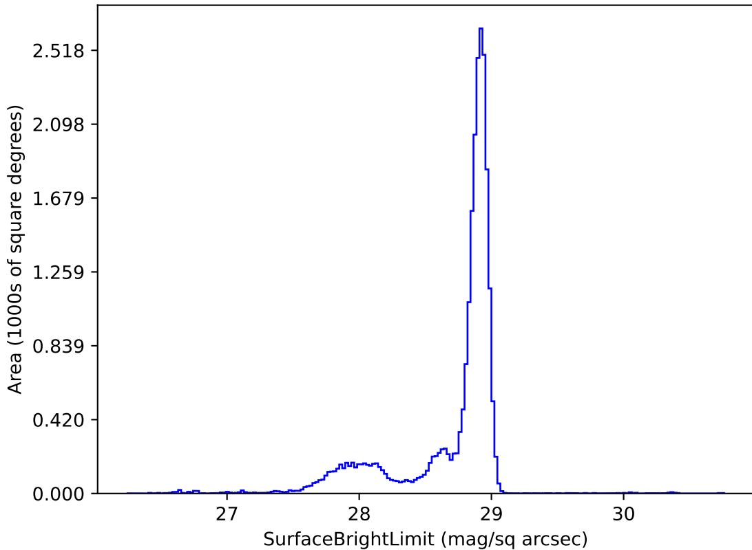
baseline_v3.3_10yrs u: SurfaceBrightLimit
