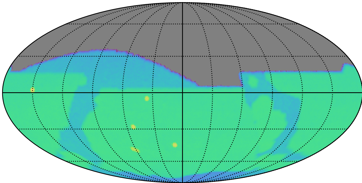
baseline_v3.3_10yrs r: SurfaceBrightLimit
