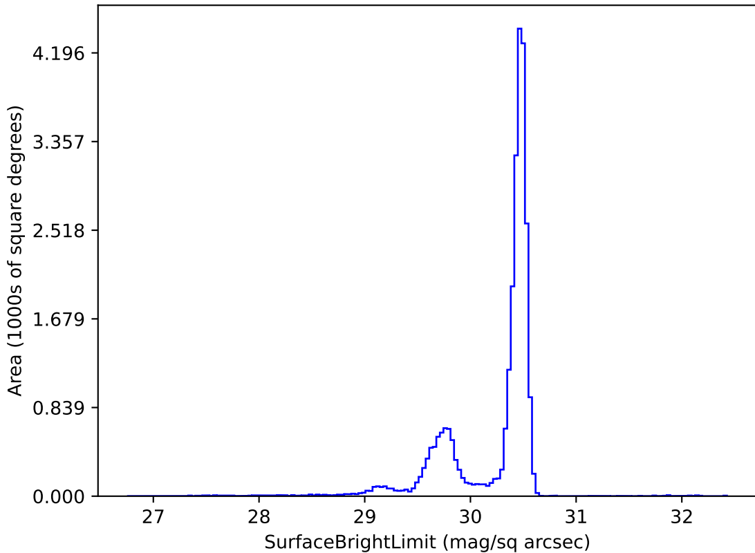
baseline_v3.3_10yrs r: SurfaceBrightLimit
