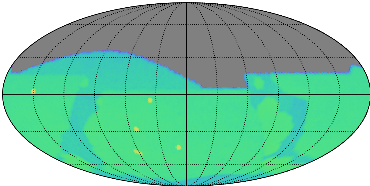
baseline_v3.3_10yrs g: SurfaceBrightLimit
