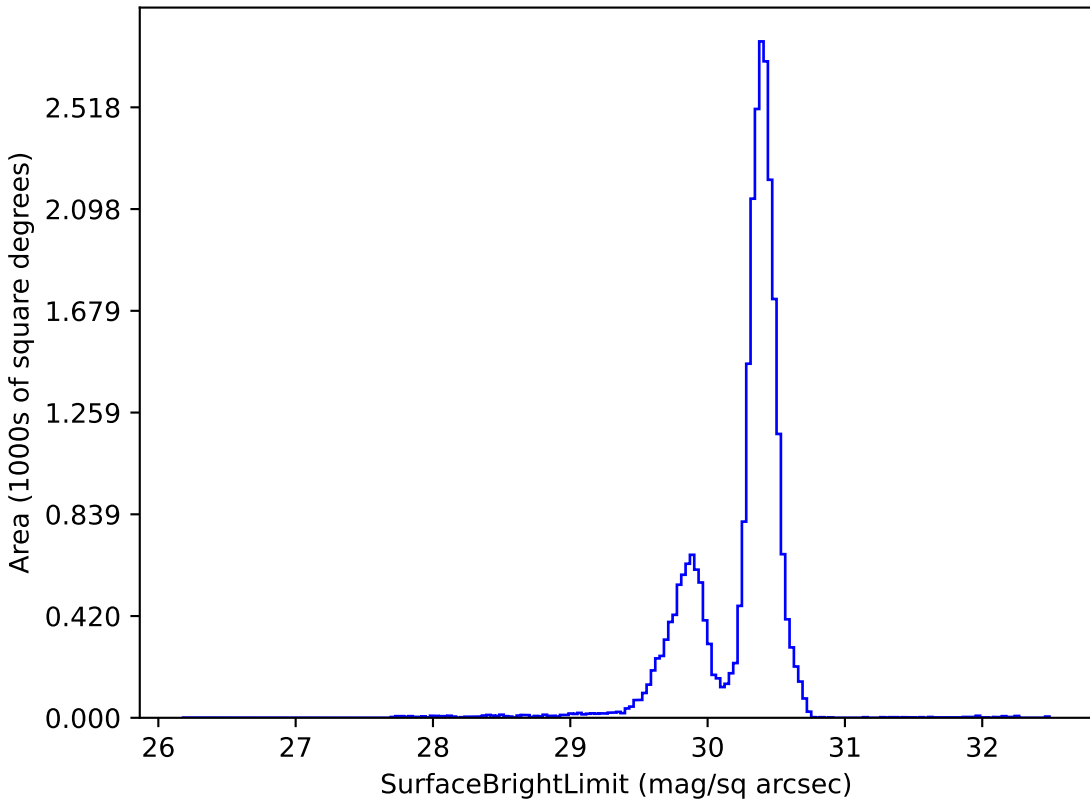
baseline_v3.3_10yrs g: SurfaceBrightLimit
