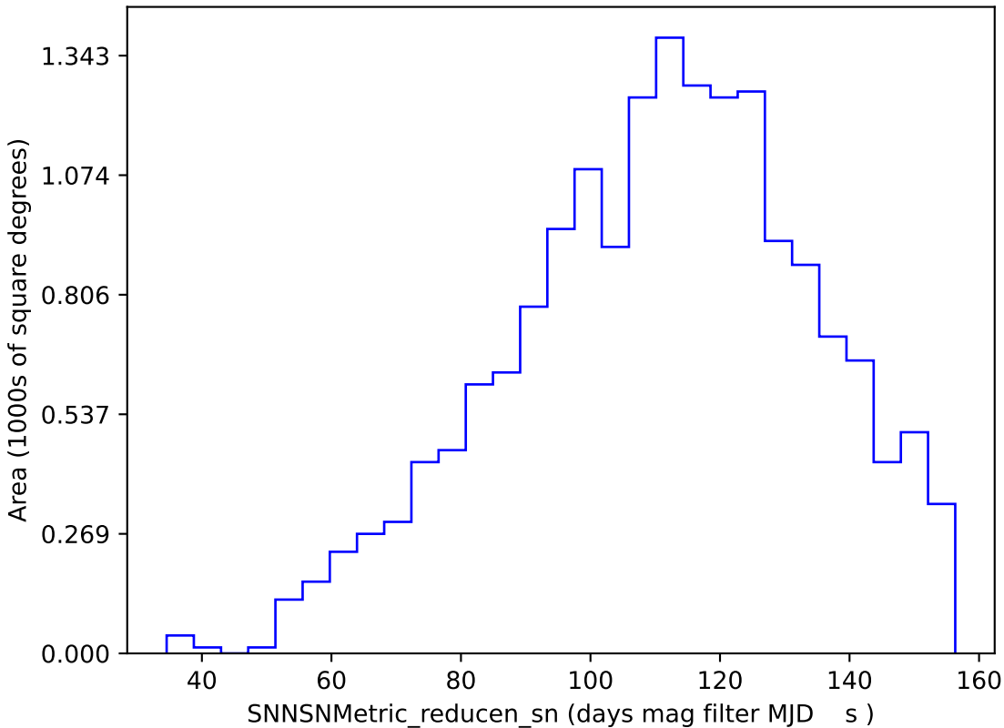
baseline_v3.3_10yrs DDF excluded: SNNSNMetric_reducen_sn
