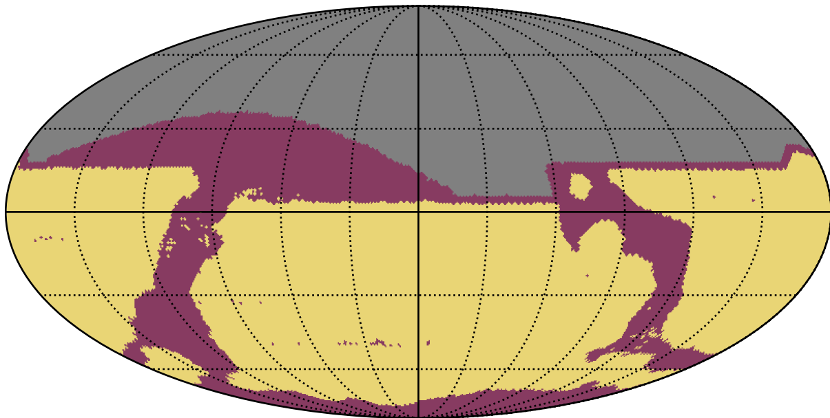
baseline_v3.3_10yrs : RapidRevisits
