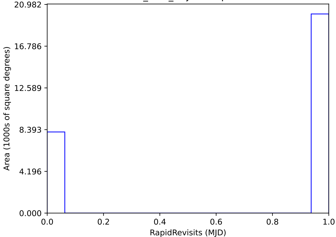
baseline_v3.3_10yrs : RapidRevisits
