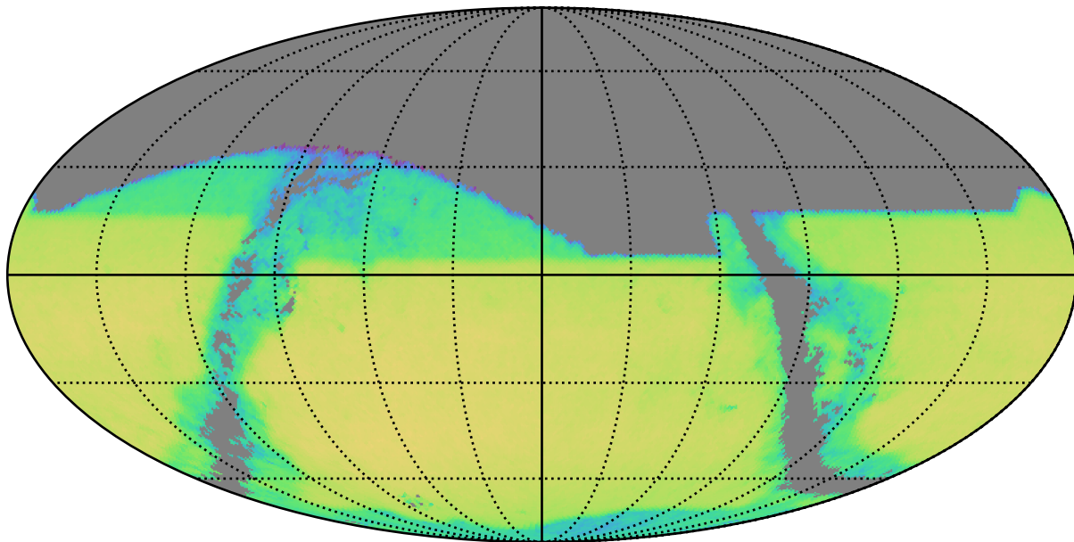
baseline_v3.3_10yrs z band and non-DD: QSONumberCountsMetric
