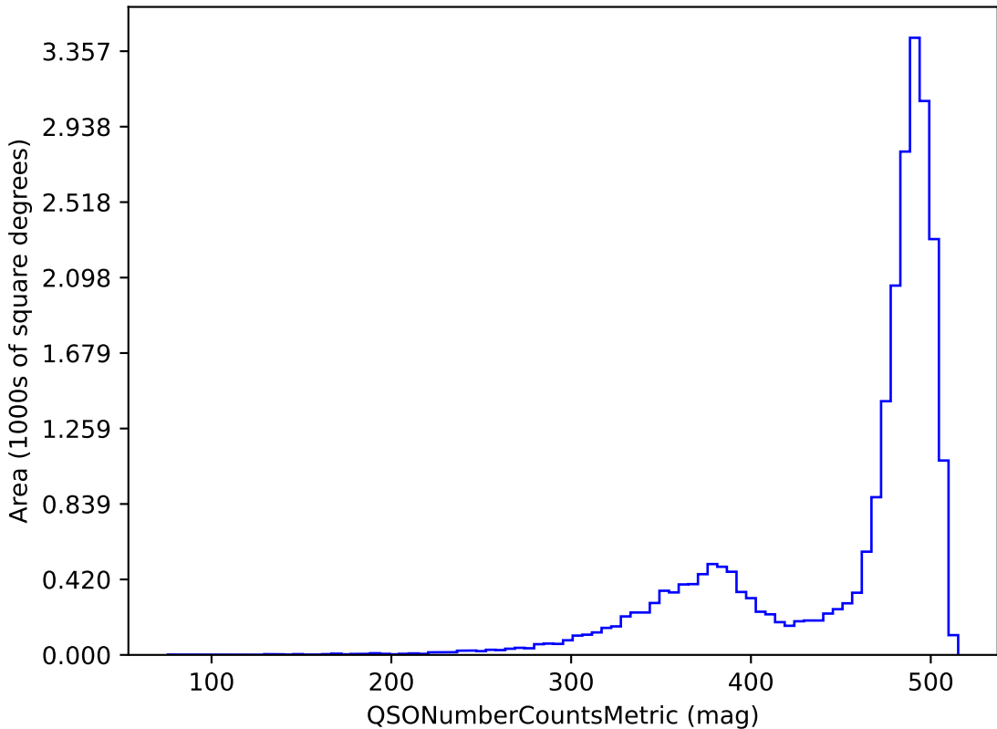
baseline_v3.3_10yrs z band and non-DD: QSONumberCountsMetric
