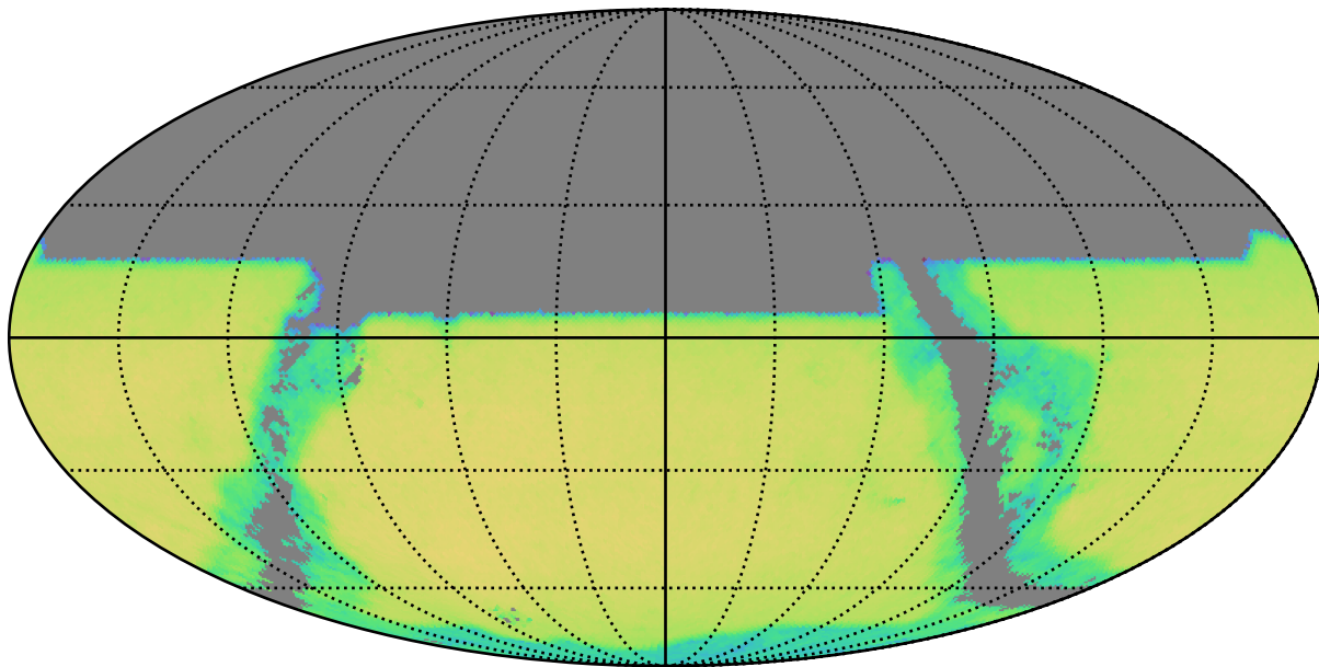
baseline_v3.3_10yrs y band and non-DD: QSONumberCountsMetric
