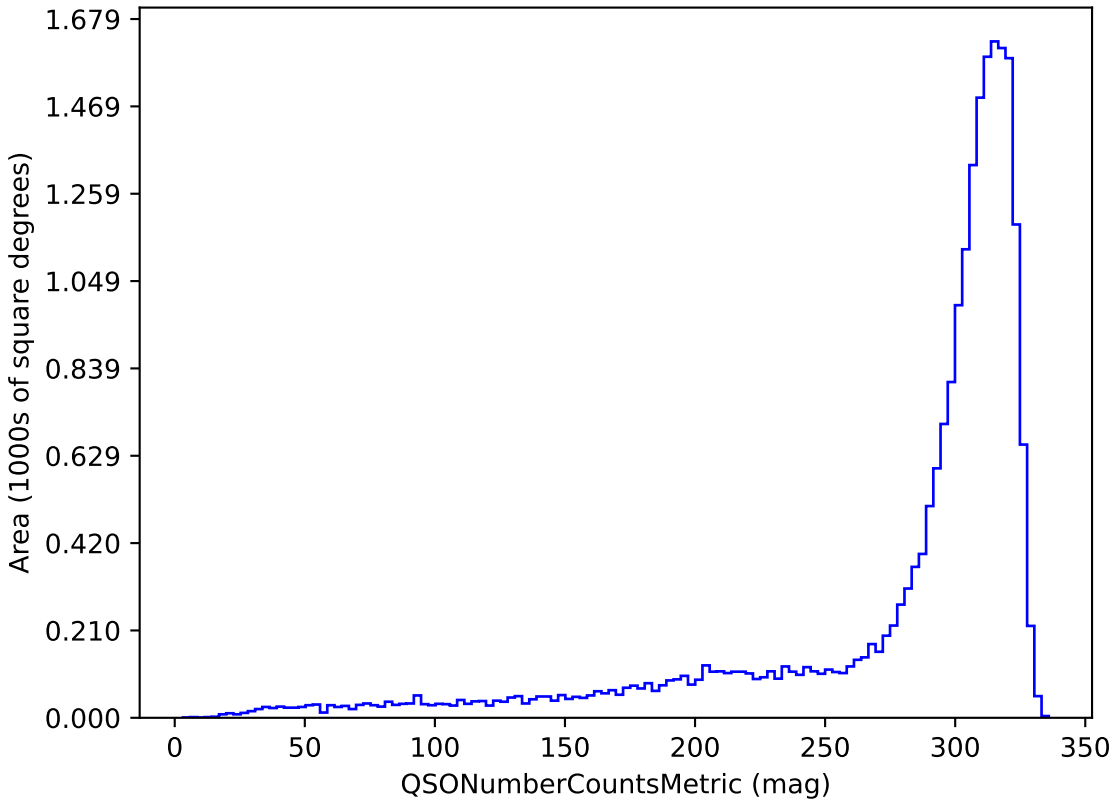
baseline_v3.3_10yrs u band and non-DD: QSONumberCountsMetric
