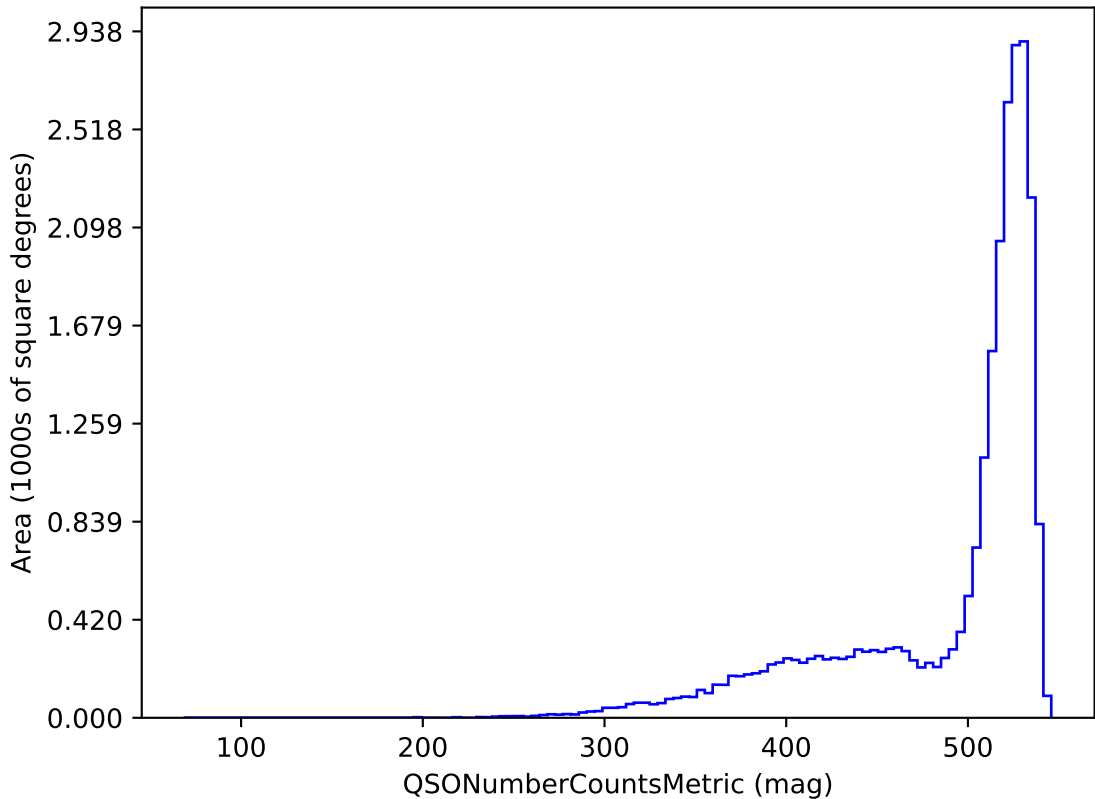
baseline_v3.3_10yrs r band and non-DD: QSONumberCountsMetric
