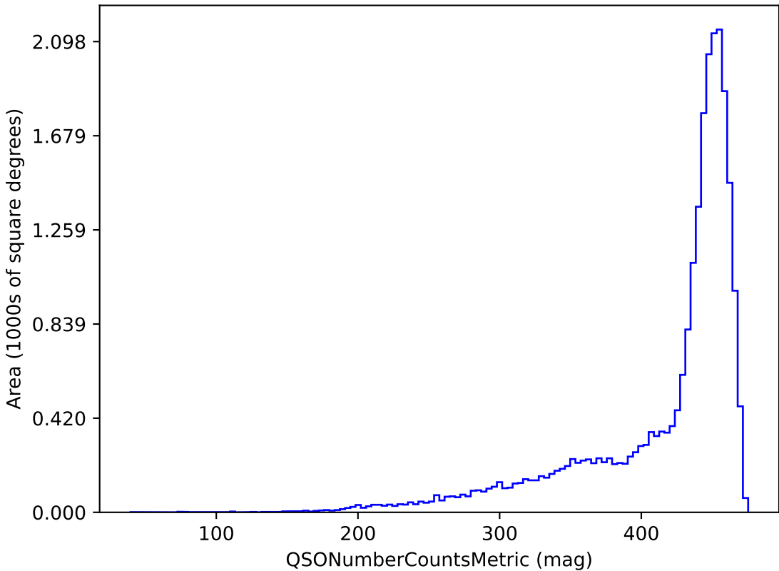
baseline_v3.3_10yrs g band and non-DD: QSONumberCountsMetric
