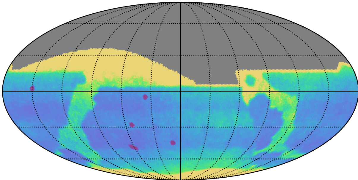
baseline_v3.3_10yrs : Proper Motion Uncert @ 24.0
