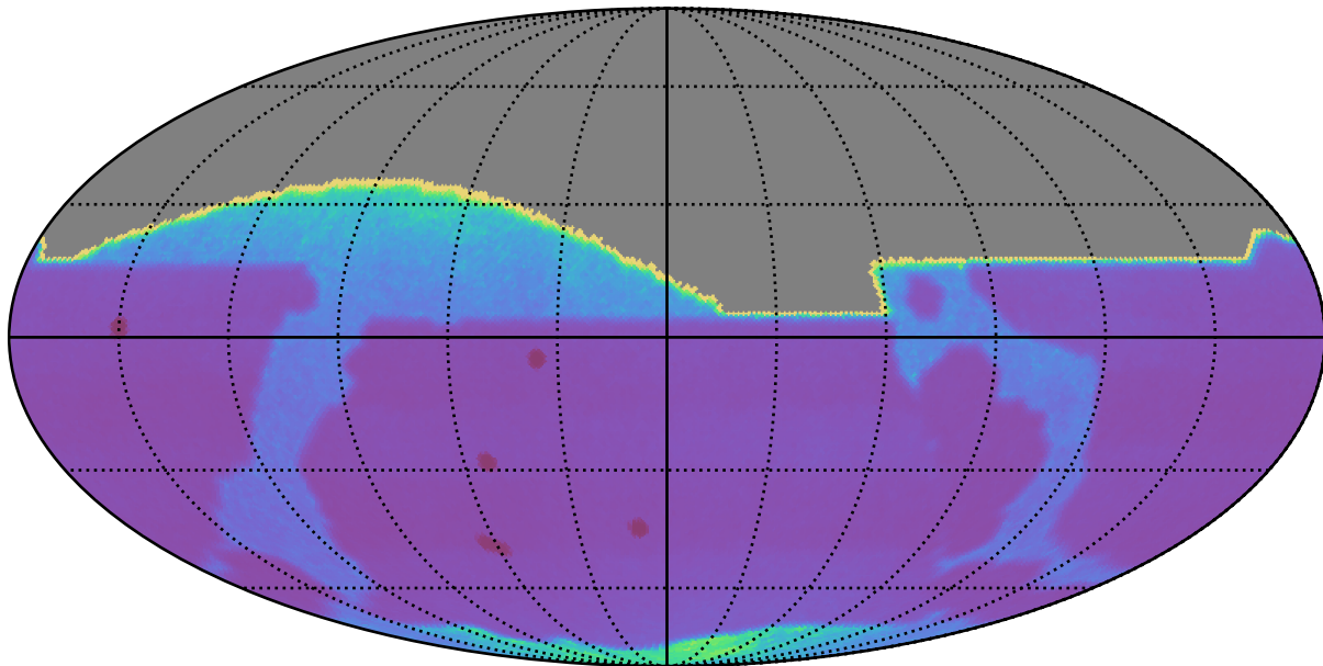
baseline_v3.3_10yrs : Proper Motion Uncert @ 20.5
