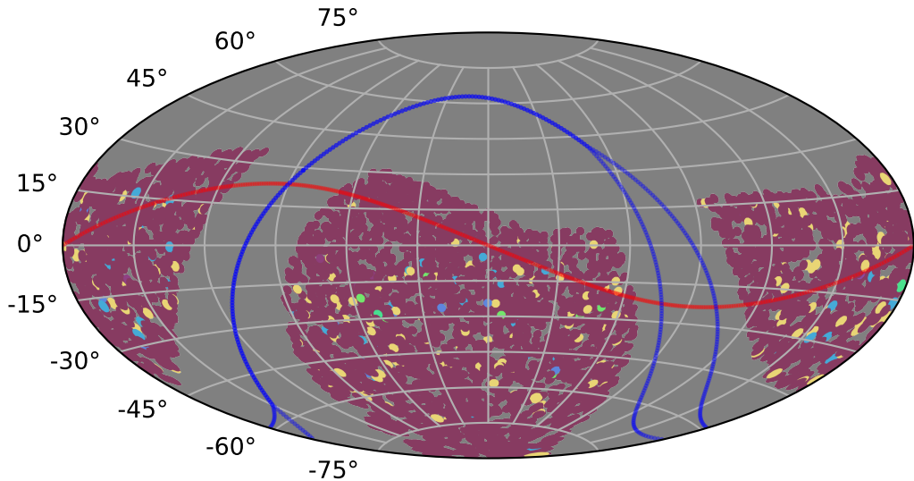
baseline_v3.3_10yrs : PrestoKNe_score_p
