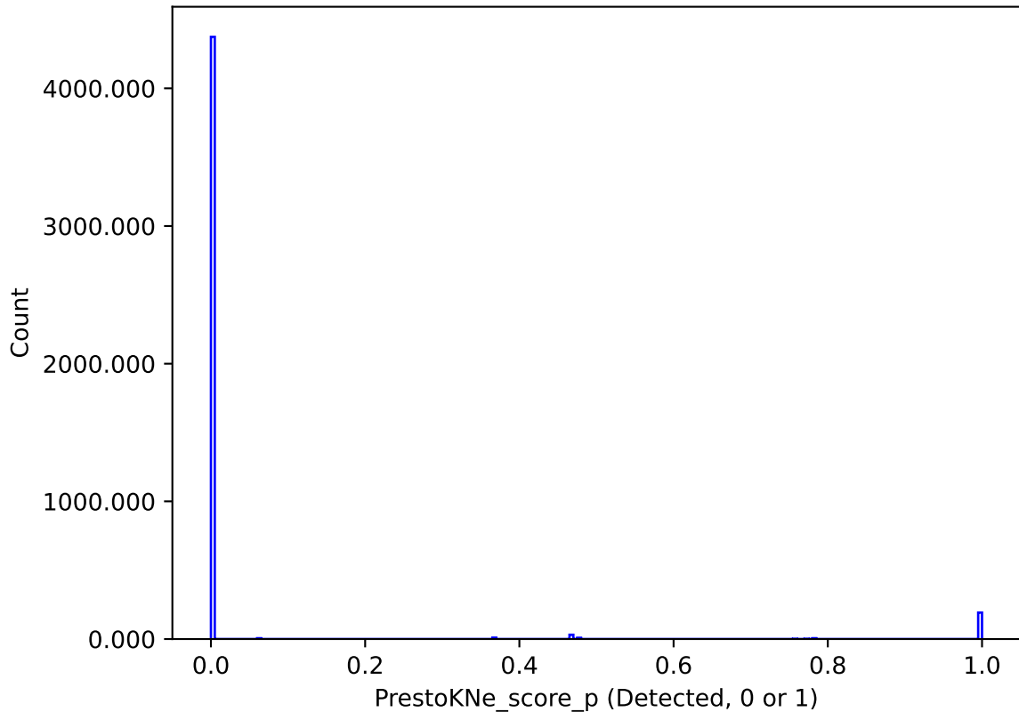
baseline_v3.3_10yrs : PrestoKNe_score_p
