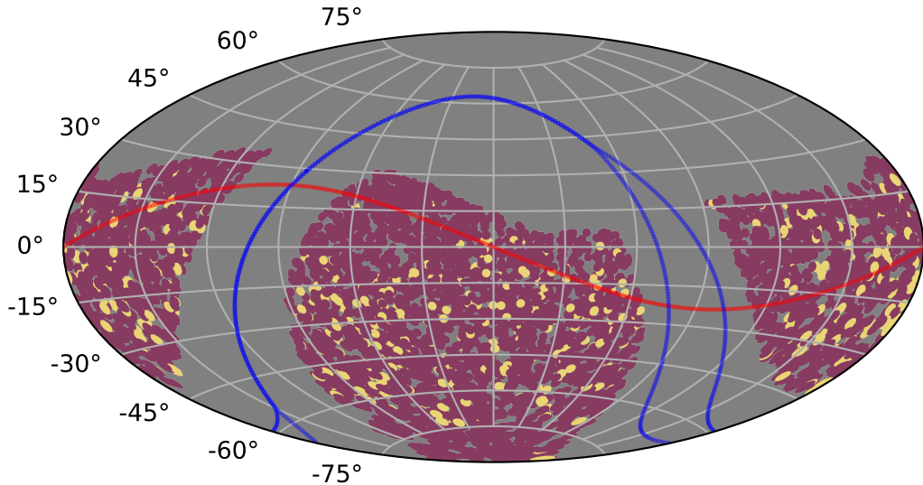
baseline_v3.3_10yrs : PrestoKNe_presto_color_detect
