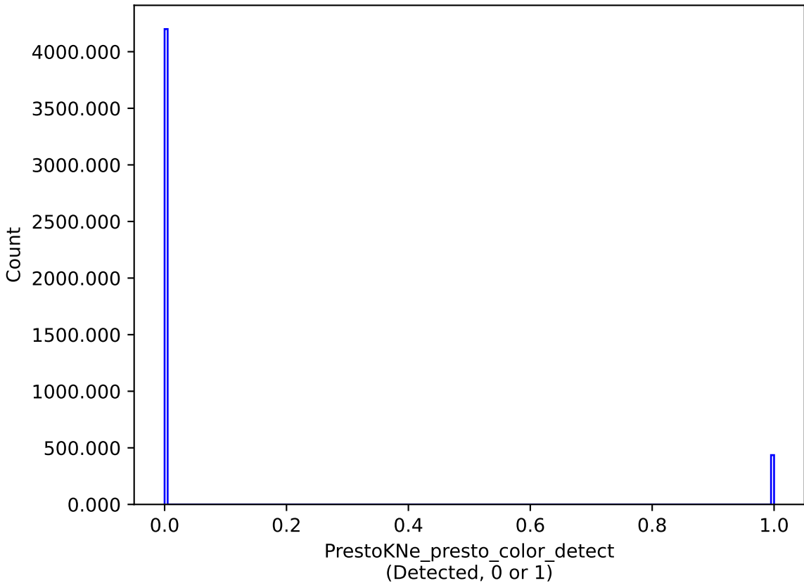
baseline_v3.3_10yrs : PrestoKNe_presto_color_detect
