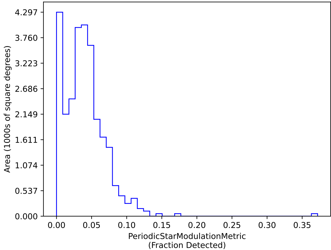
baseline_v3.3_10yrs dm 21 interval 30 R Rc Year 1-2: PeriodicStarModulationMetric
