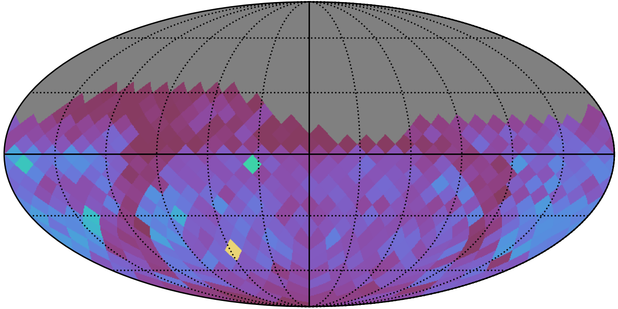
baseline_v3.3_10yrs dm 20 interval 30 RRC Year 1-2: PeriodicStarModulationMetric
