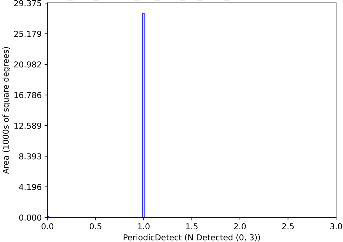
baseline_v3.3_10yrs P_2.0_Mag_24_Amp_0.05-0.1-1: PeriodicDetect
