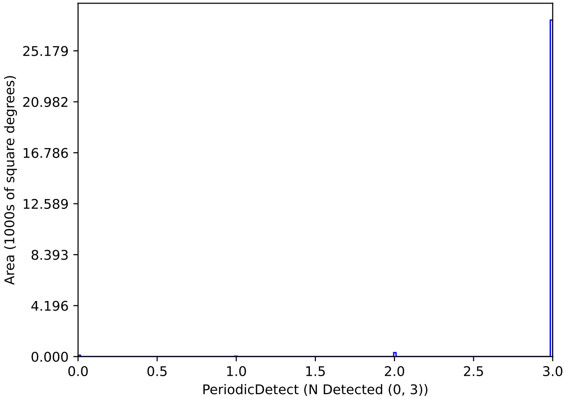
baseline_v3.3_10yrs P_2.0_Mag_21_Amp_0.05-0.1-1: PeriodicDetect
