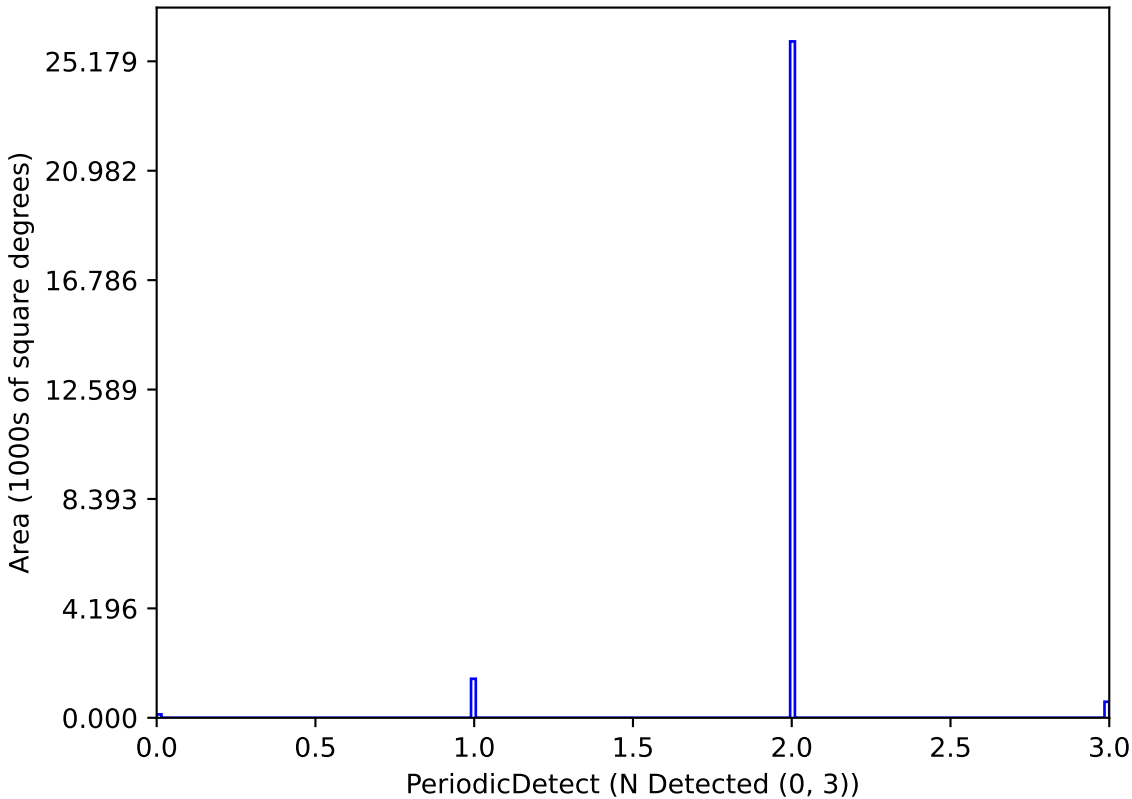
baseline_v3.3_10yrs P_1.0_Mag_21_Amp_0.05-0.1-1: PeriodicDetect
