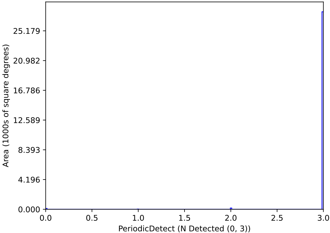
baseline_v3.3_10yrs P_0.5_Mag_21_Amp_0.05-0.1-1: PeriodicDetect
