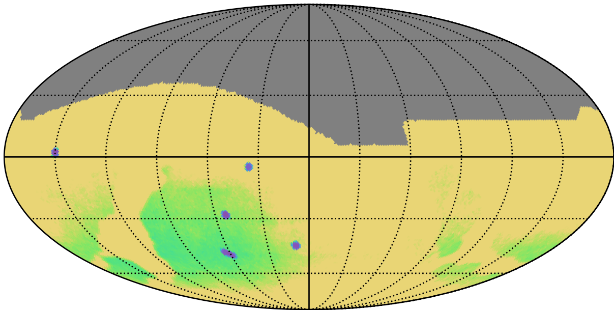
baseline_v3.3_10yrs : Parallax Uncert @ 22.4
