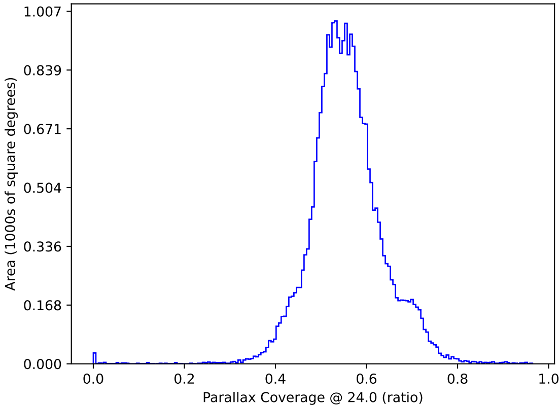
baseline_v3.3_10yrs : Parallax Coverage @ 24.0
