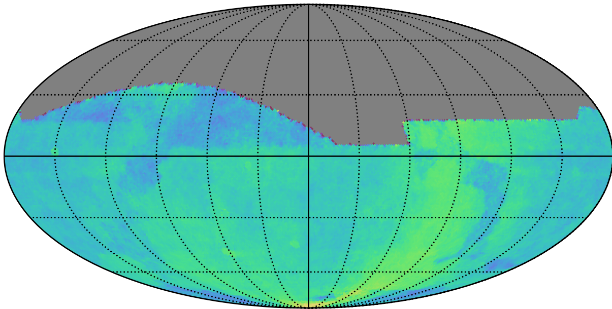
baseline_v3.3_10yrs : Parallax Coverage @ 22.4
