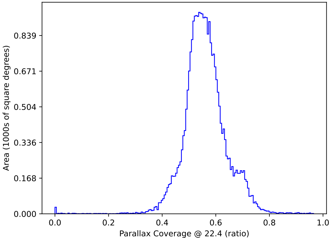
baseline_v3.3_10yrs : Parallax Coverage @ 22.4
