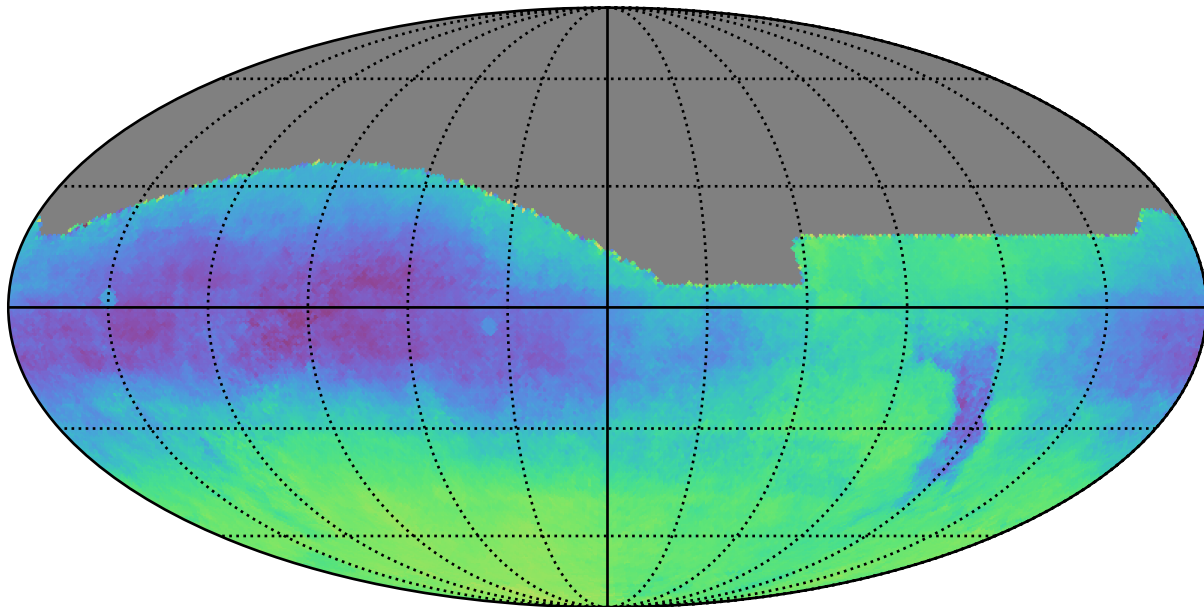
baseline_v3.3_10yrs : Parallax-DCR degeneracy @ 24.0
