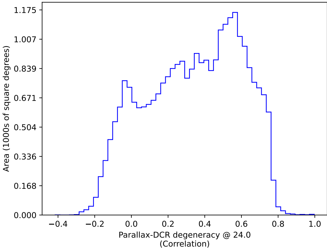
baseline_v3.3_10yrs : Parallax-DCR degeneracy @ 24.0
