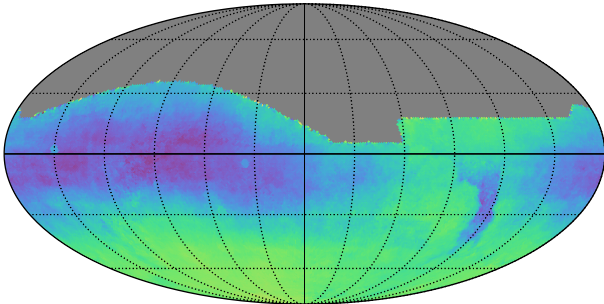
baseline_v3.3_10yrs : Parallax-DCR degeneracy @ 22.4
