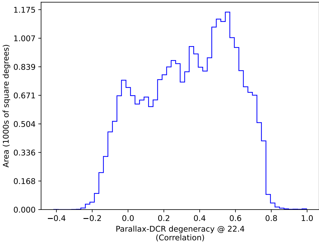
baseline_v3.3_10yrs : Parallax-DCR degeneracy @ 22.4
