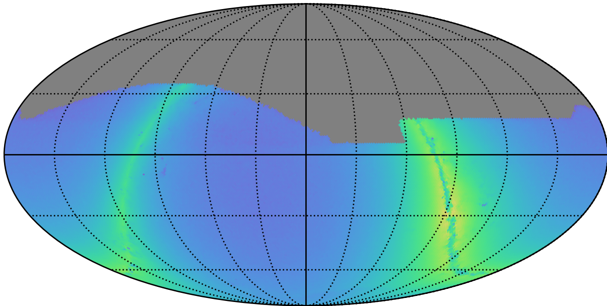
baseline_v3.3_10yrs z: Nstars_no_crowding
