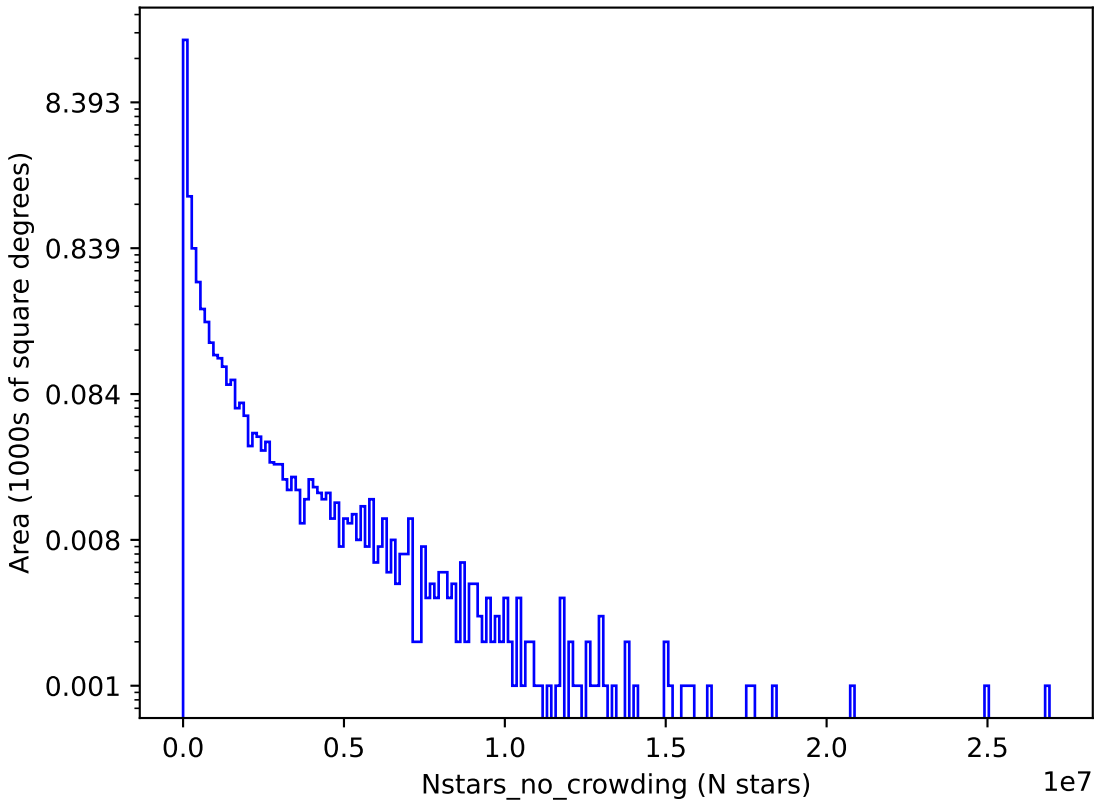
baseline_v3.3_10yrs z: Nstars_no_crowding
