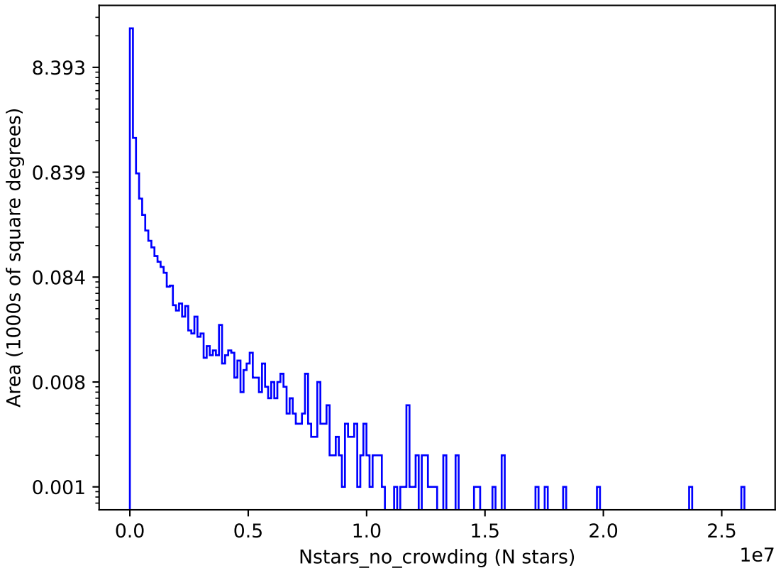
baseline_v3.3_10yrs y: Nstars_no_crowding
