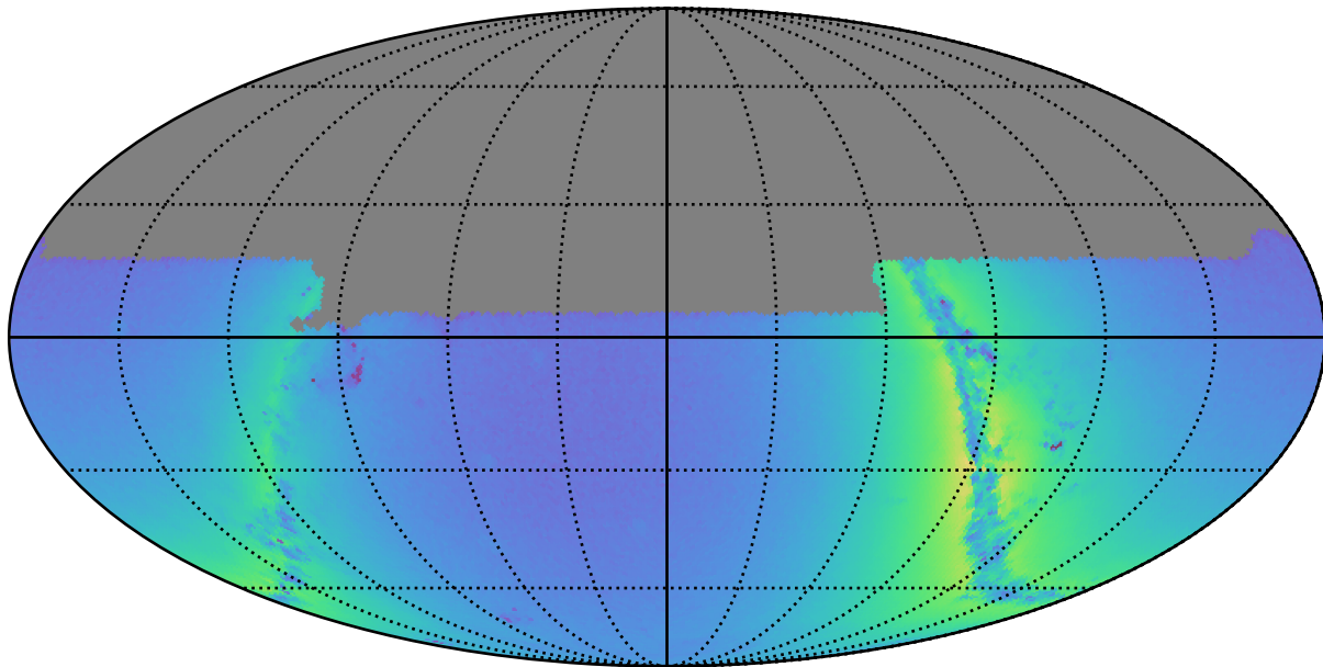
baseline_v3.3_10yrs u: Nstars_no_crowding
