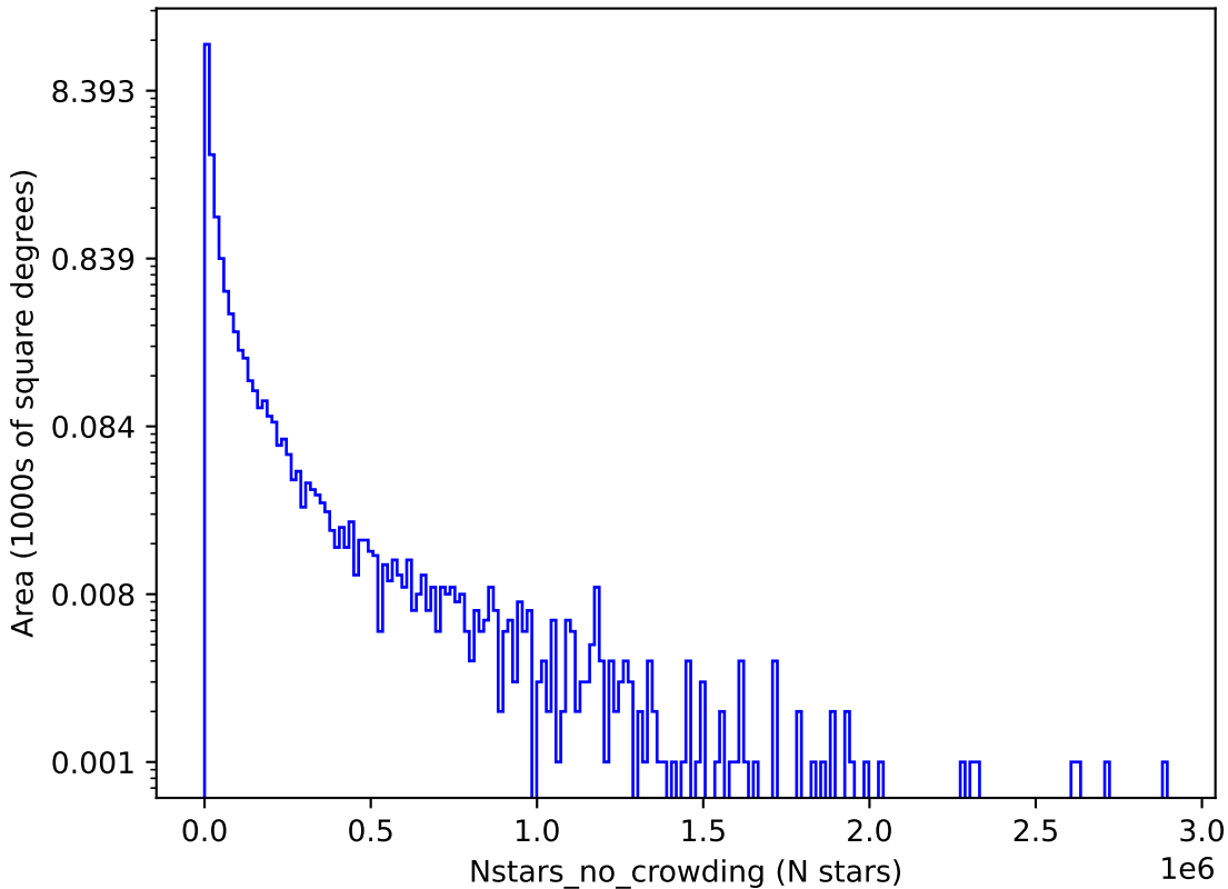
baseline_v3.3_10yrs u: Nstars_no_crowding
