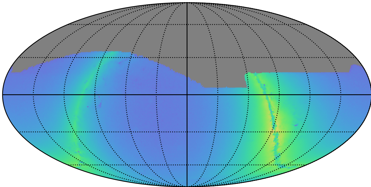
baseline_v3.3_10yrs r: Nstars_no_crowding
